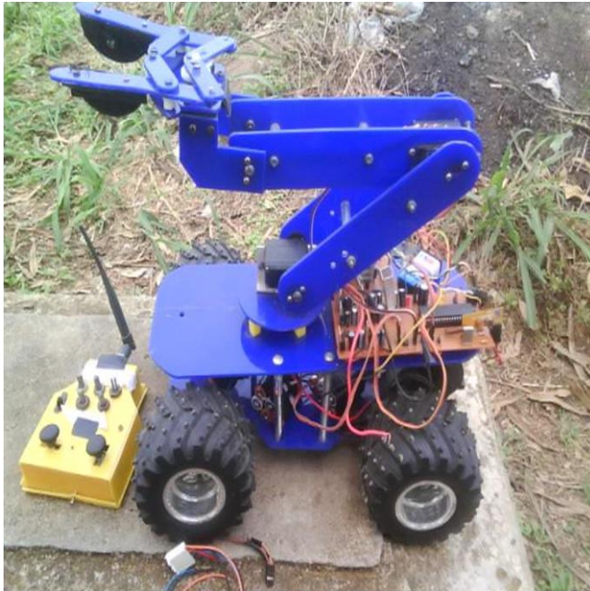
Plate 1: GSM/RF-based Controlled Robotic Car
