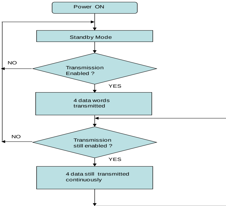
Fig 5: Flow Chart of the Developed CCS Software Algorithm
