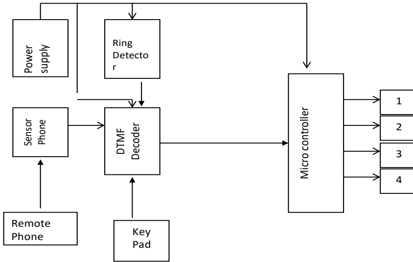
Fig.6: Embedded Systems Design Block Diagram of the GSM-based Controlled System (GbCS)
